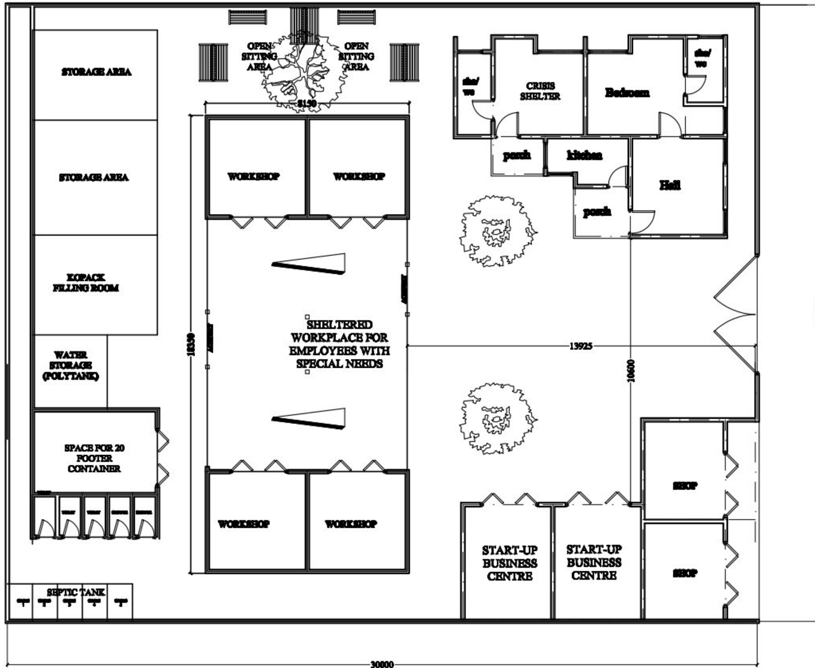
BLOCK PLAN
